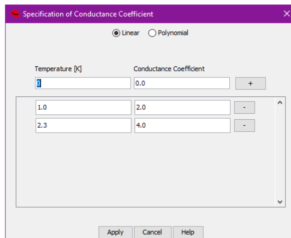
Figure 20 : Linear model for conductance
