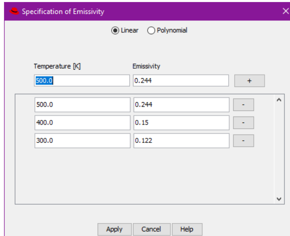
Figure 49 Entry of a linear evaluation
