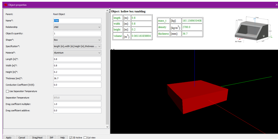
Figure 19 Adding an object window.
