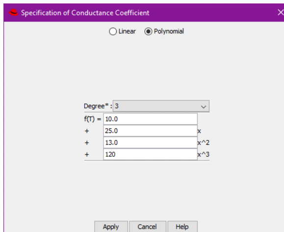
Figure 21 : Polynomial model for conductance
