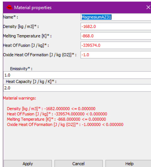
Figure 47 Adding a customised material.
