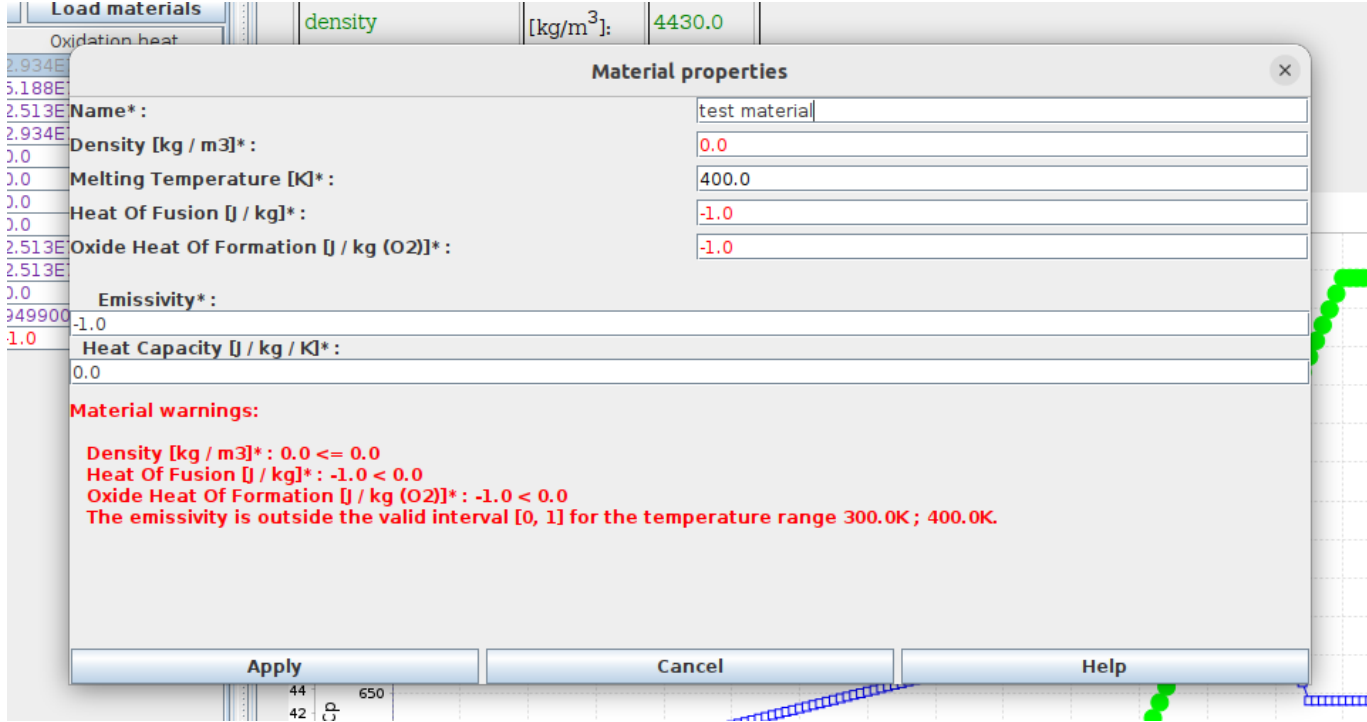
Figure 67 Entry of a user-defined material
