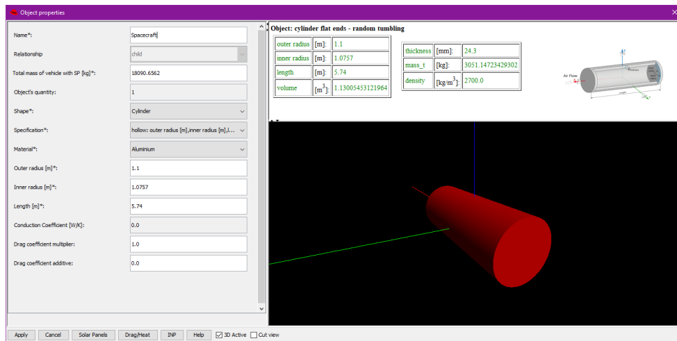
Figure 18 Adding a root object window.
