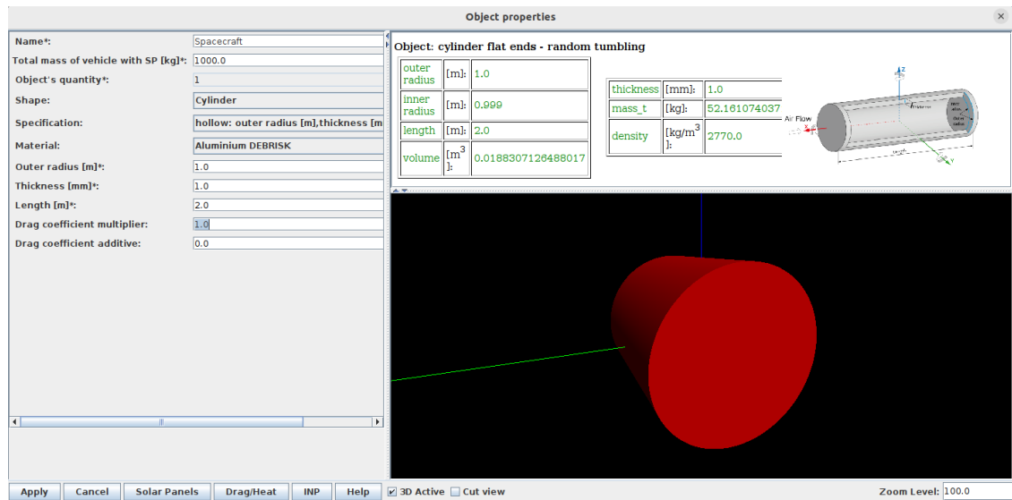
Figure 75 Creating a spacecraft.
